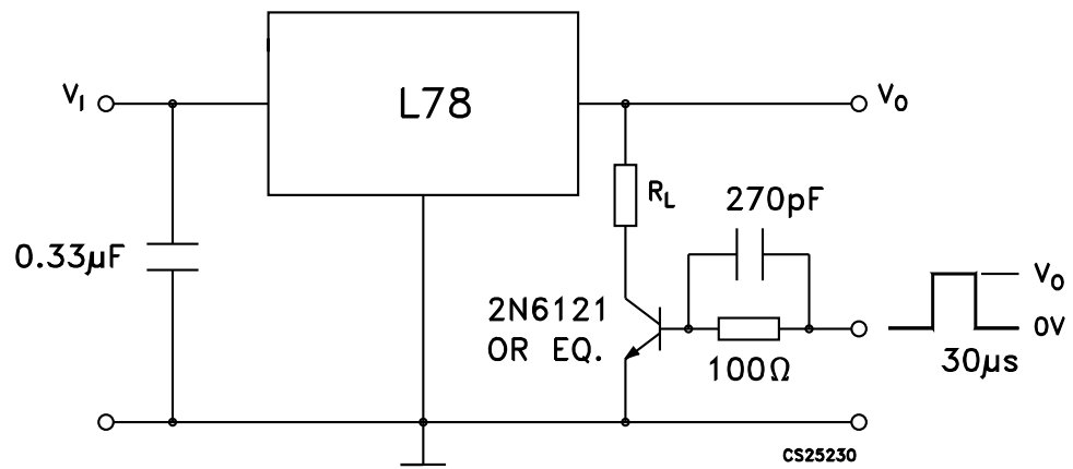
Figure 7. Load regulation
