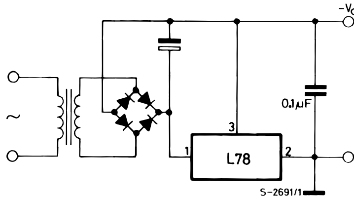
Figure 18. Negative output voltage circuit
