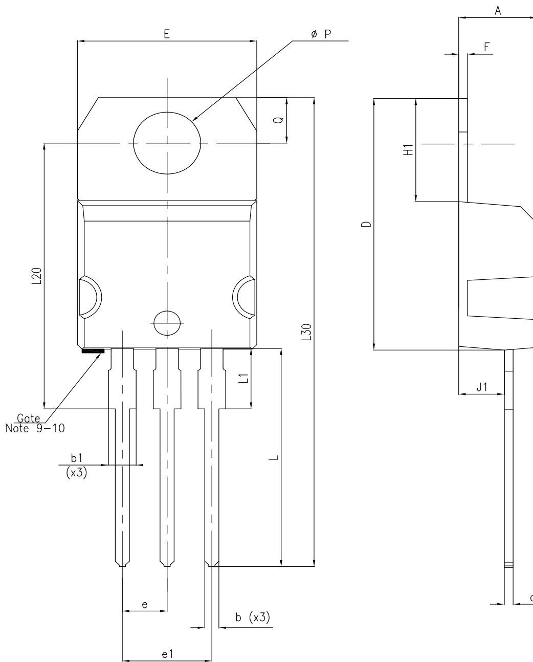
Figure 39. TO-220 (single gauge) package outline
