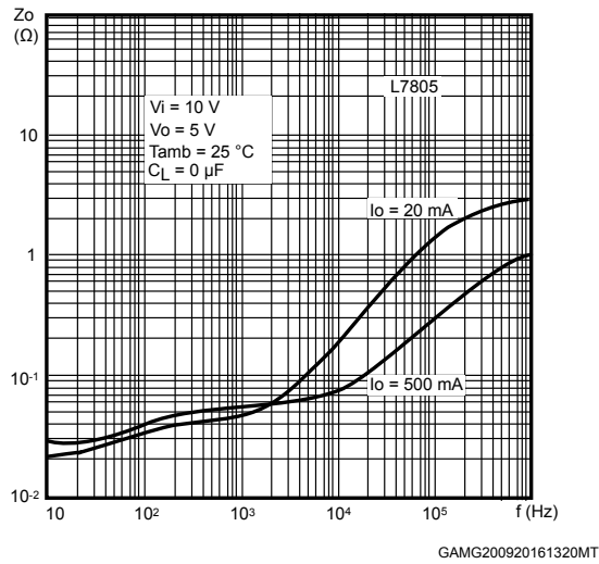
Figure 33. Output impedance vs frequency
