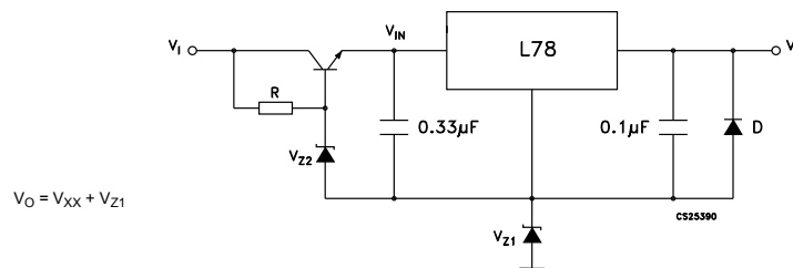
Figure 22. High input and output voltage
