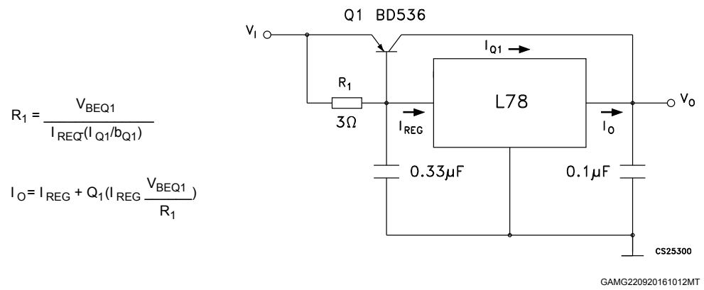
Figure 15. High output current with short circuit protection
