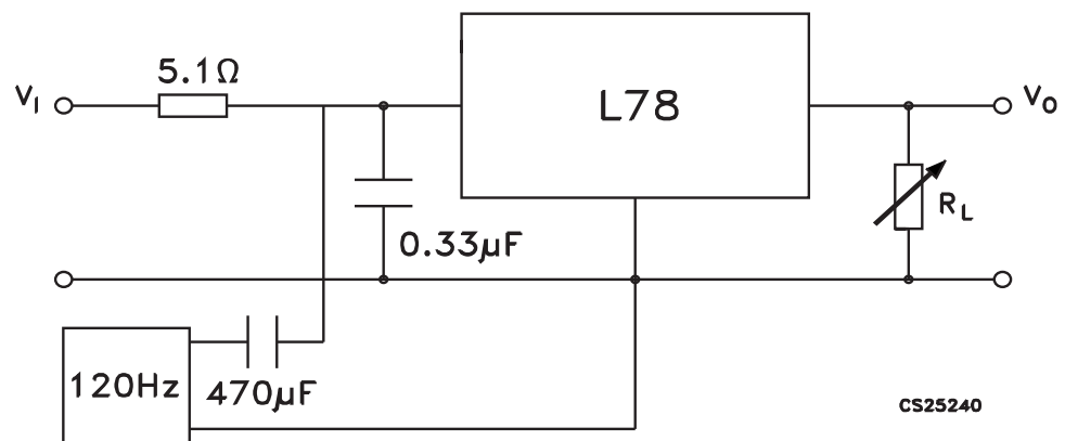
Figure 8. Ripple rejection
