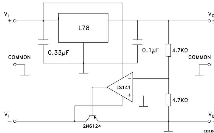
Figure 16. Tracking voltage regulator
