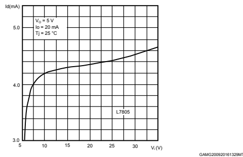
Figure 37. Quiescent current vs. input voltage
