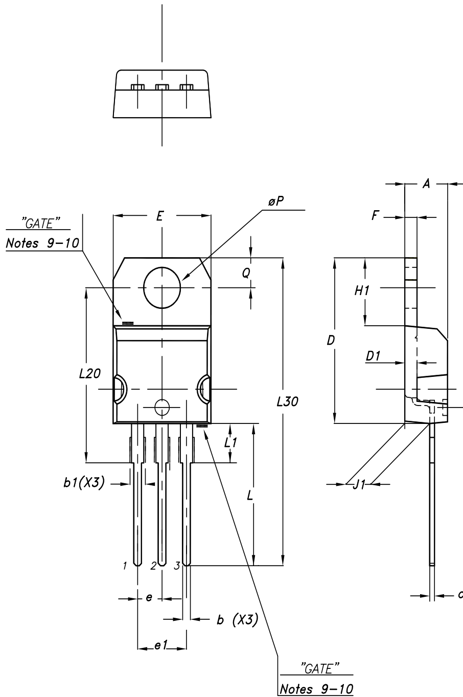
Figure 38. TO-220 (dual gauge) package outline
