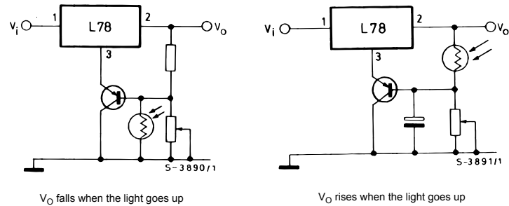
Figure 27. Light controllers ( V_{O(\min)} = V_{XX} + V_{BE} )
