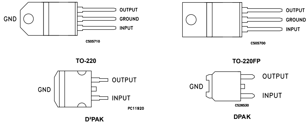
Figure 3. Pin connections (top view)
