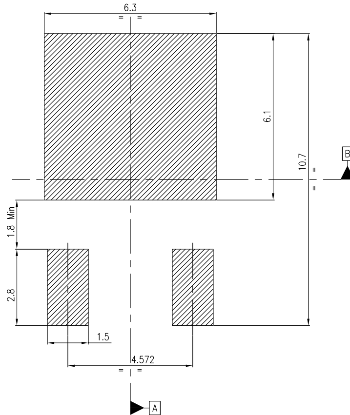
Figure 44. DPAK recommended footprint (dimensions are in mm)
