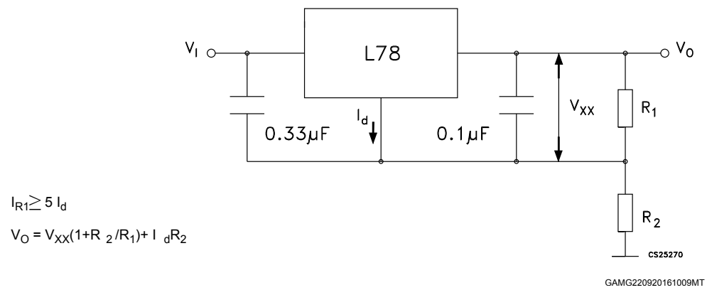
Figure 12. Adjustable output regulator (7 to 30 V)
