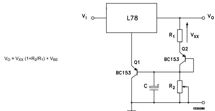
Figure 26. Adjustable output voltage with temperature compensation
