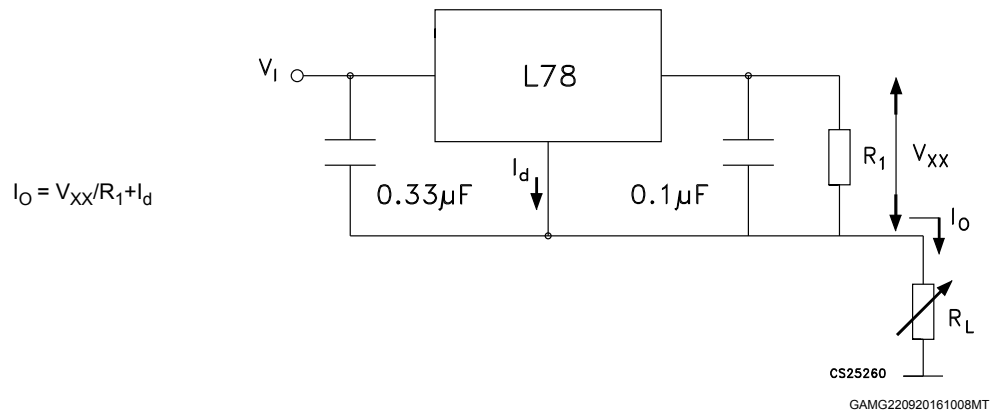
Figure 11. Circuit for increasing output voltage
