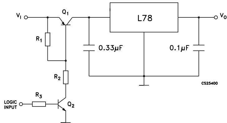
Figure 24. Remote shutdown
