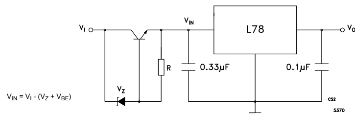
Figure 20. High input voltage circuit (configuration 1)
