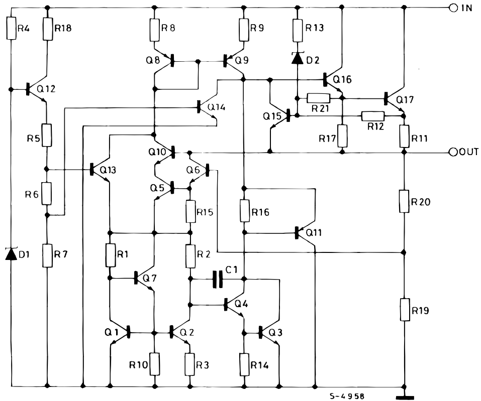
Figure 4. Schematic diagram
