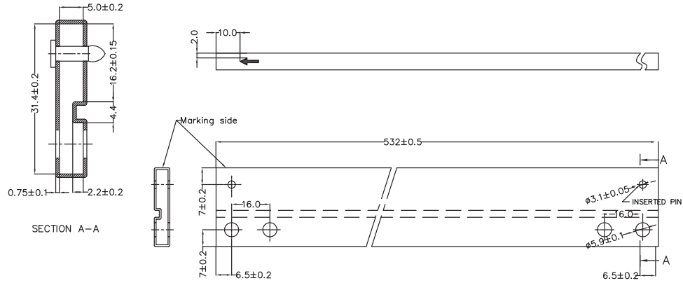
Figure 42. Tube for TO-220 (single gauge) (mm.)
