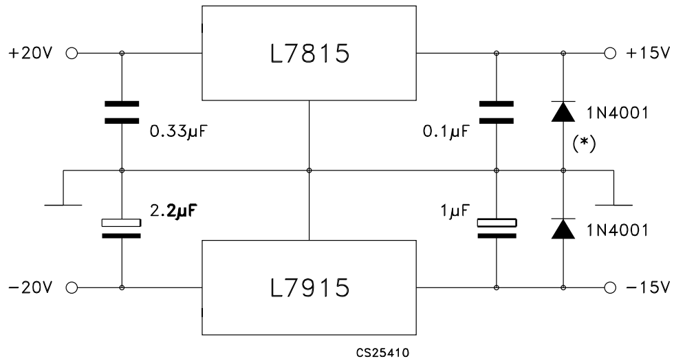
Figure 17. Split power supply ( \pm 15 V - 1 A)
