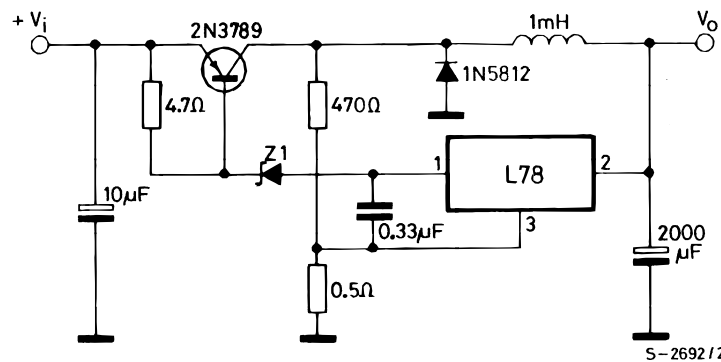
Figure 20. High input voltage circuit (configuration 1)
