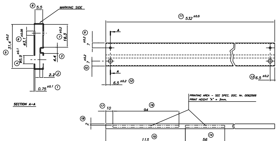
Figure 41. Tube for TO-220 (dual gauge) (mm.)
