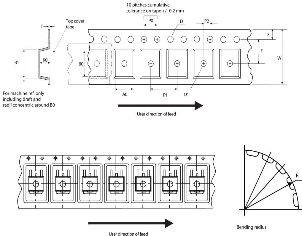
Figure 48. Tape outline
