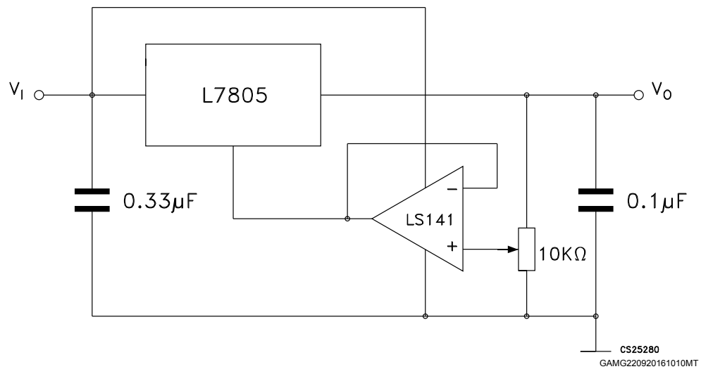
Figure 12. Adjustable output regulator (7 to 30 V)
