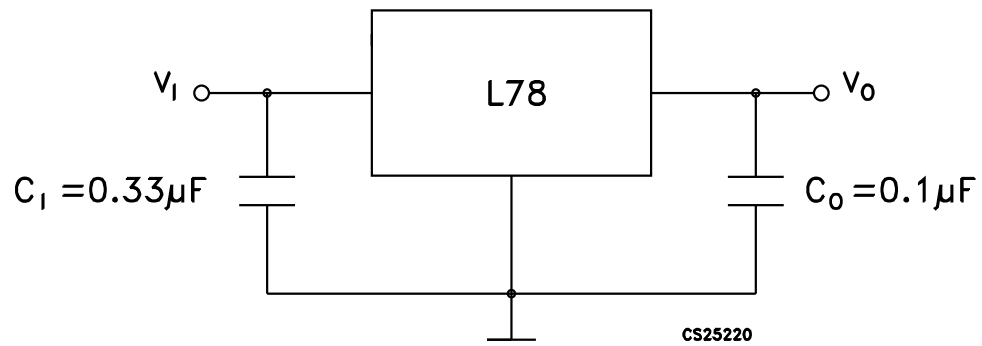
Figure 5. Application circuits
