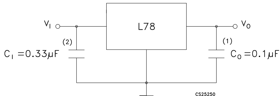
Figure 9. Fixed output regulator
